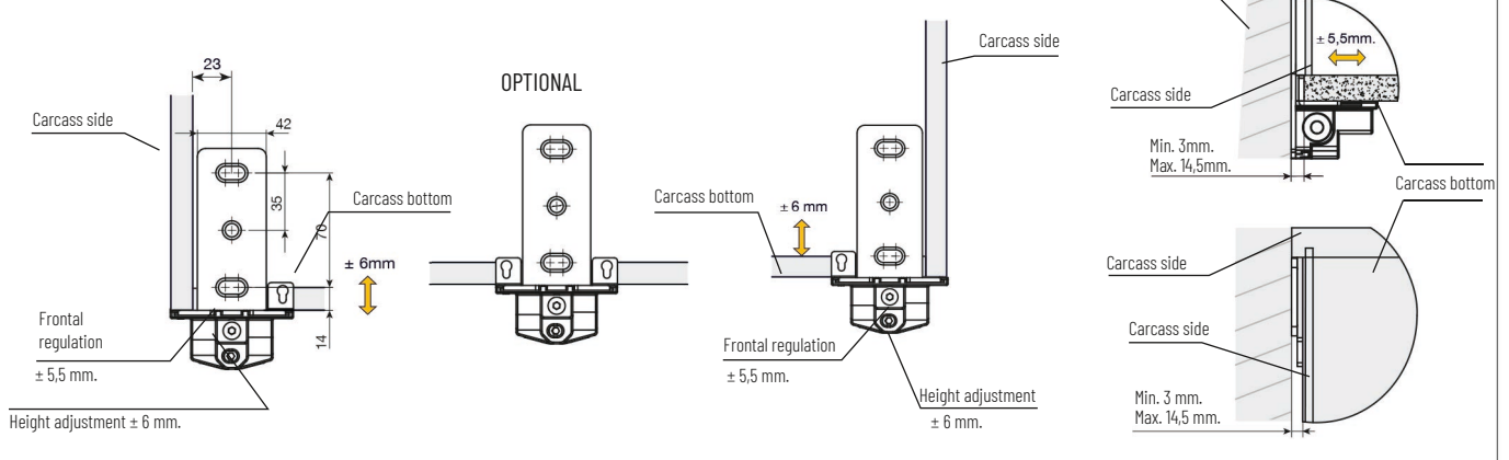
Lower support fitting 3mm.
