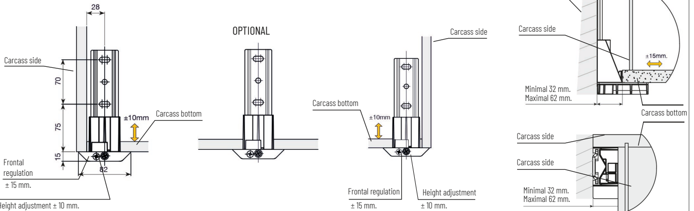
Lower support fitting 32 mm
