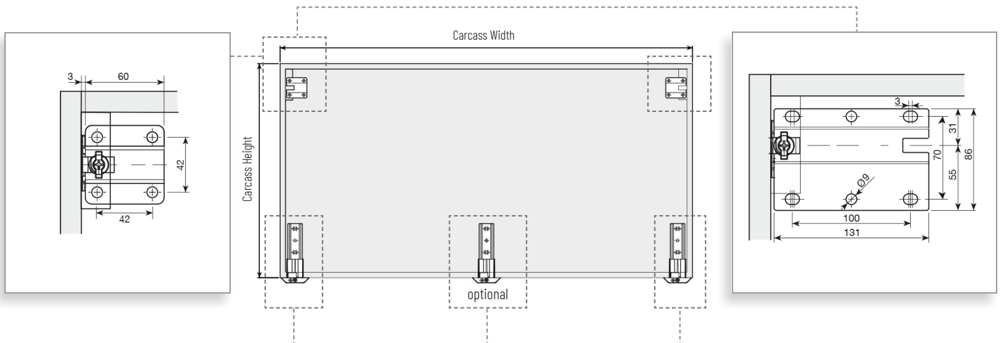
Lower support fitting 32 mm
