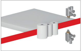
2 Glue and Pressure Zone
