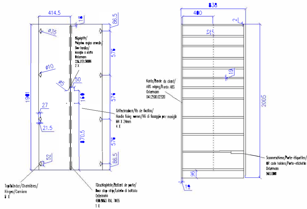
Türen/Portes/Doors/Anle
